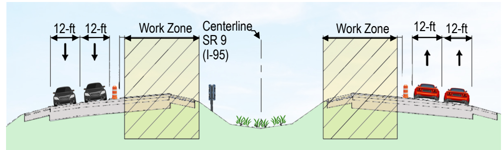
Close Inside Lanes and Resurface
