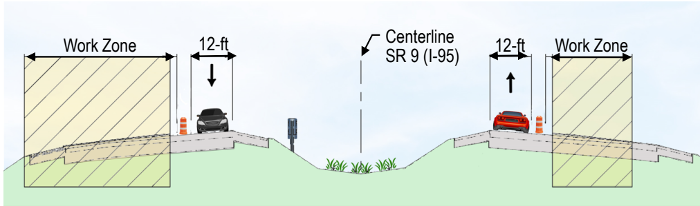
Close Outside Lanes and Resurface
